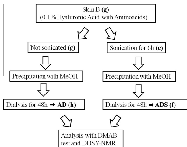
Fig. 2. The scheme of the procedure adopted for the amino acids deprivation of the samples of AAA as reported in Section . Letters are used to identify the samples.
